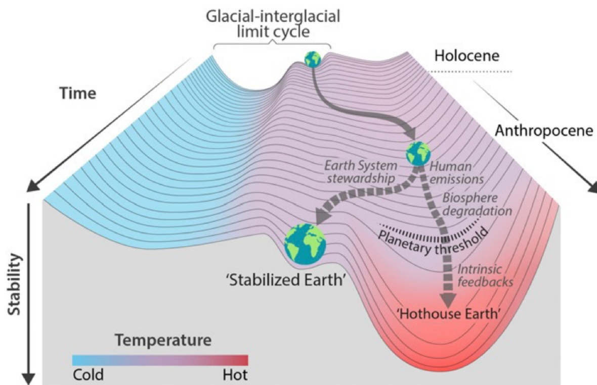
Fig. 4a: “Stability landscape showing the pathway of the Earth System out of the Holocene and thus, out of the glacial-interglacial limit cycle to its present position in the hotter Anthropocene.” Source: Steffen et al., “Trajectories of the Earth System in the Anthropocene,” 8254-8255.
