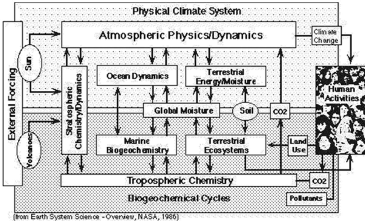
Fig. 3. The Bretherton Diagram.
